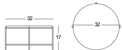
sef2531 coffee Table. overall: 32" w 32" d 17" h.
