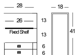
Inside Cabinet
