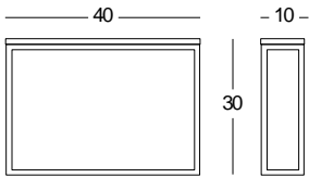
sef267 console Table. overall: 40" w 10" d 30" h.
